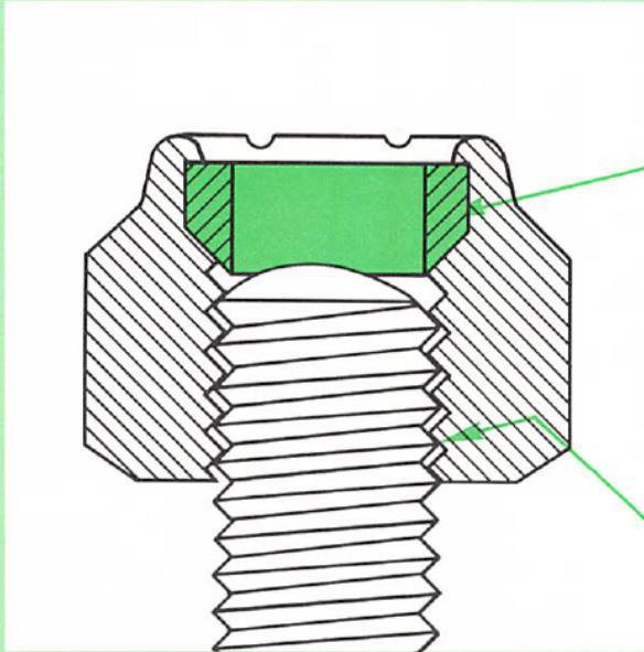
Bolt being driven into Greer nut
